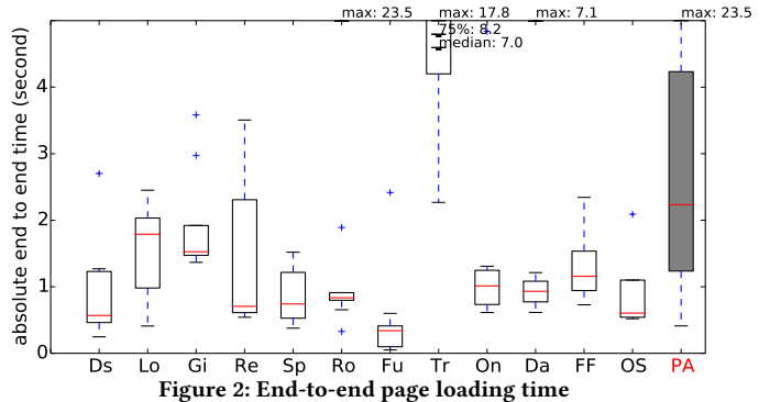
Figure 2: End-to-end page loading time Measured for top 10 time-consuming pages per application. Box: 25 to 75 percentile; Red line: median; PA: problematic actions from all 12 applications (see Section 3.2).
